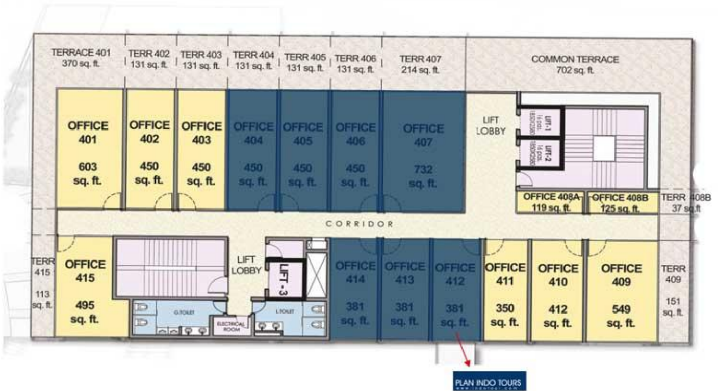
FOURTH FLOOR
